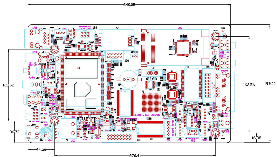
Installation dimensions of bare card M69
