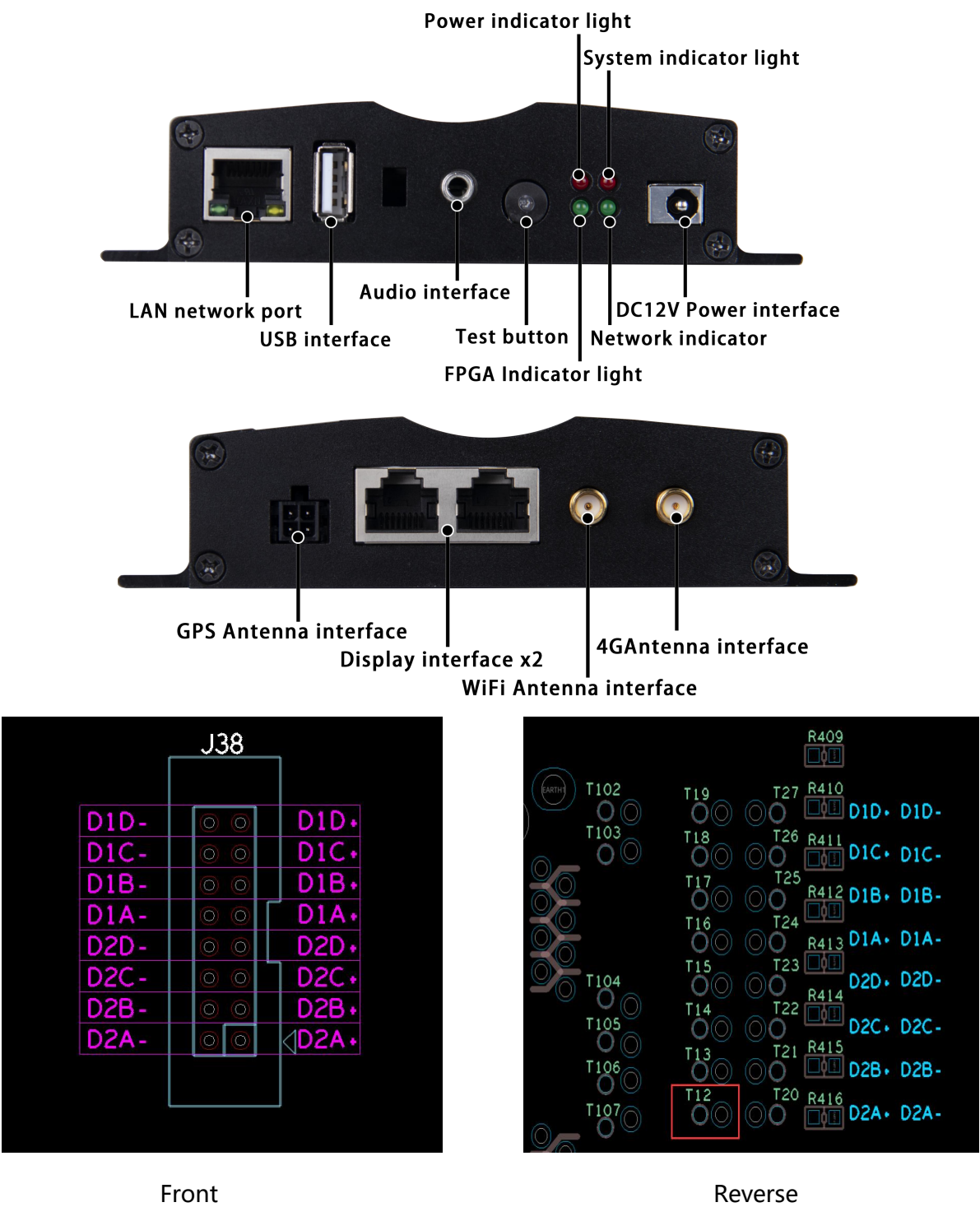
M69B Product Interface Label (with box)
