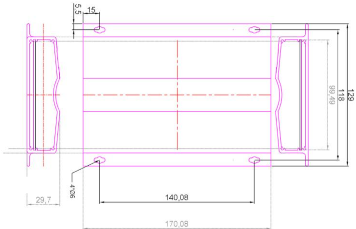
Installation dimensions of bare card M69
