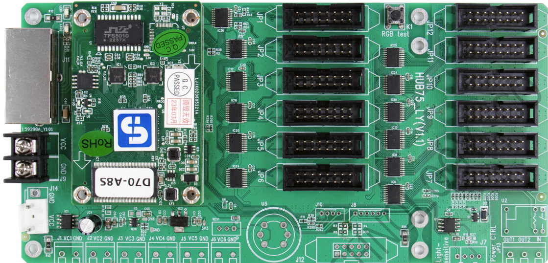
Receiver D70-A8S PRO connect with spot inspector card DJ10
