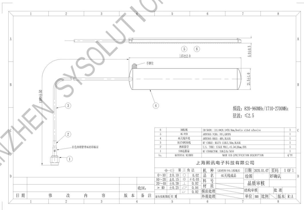
4G Patch Antenna
