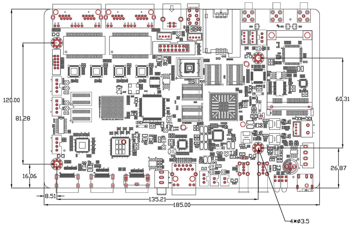
Dimensions of the M89B-S main board
