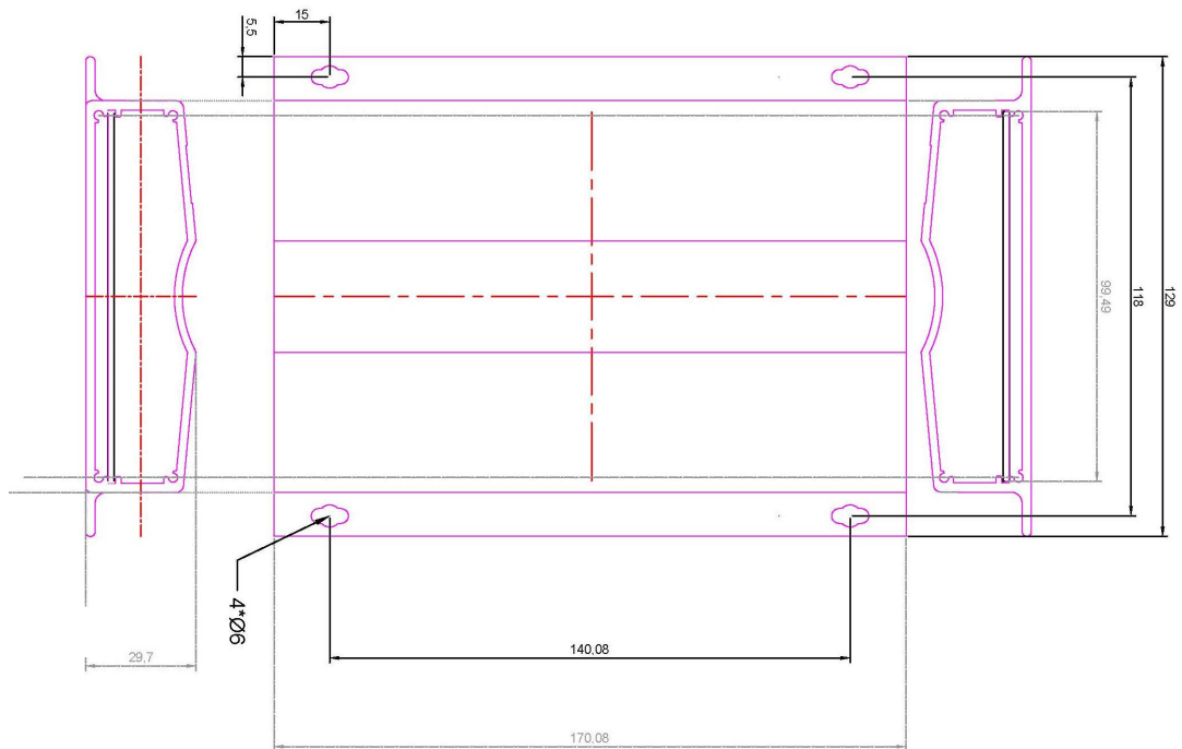
Installation dimensions of bare card M59S
