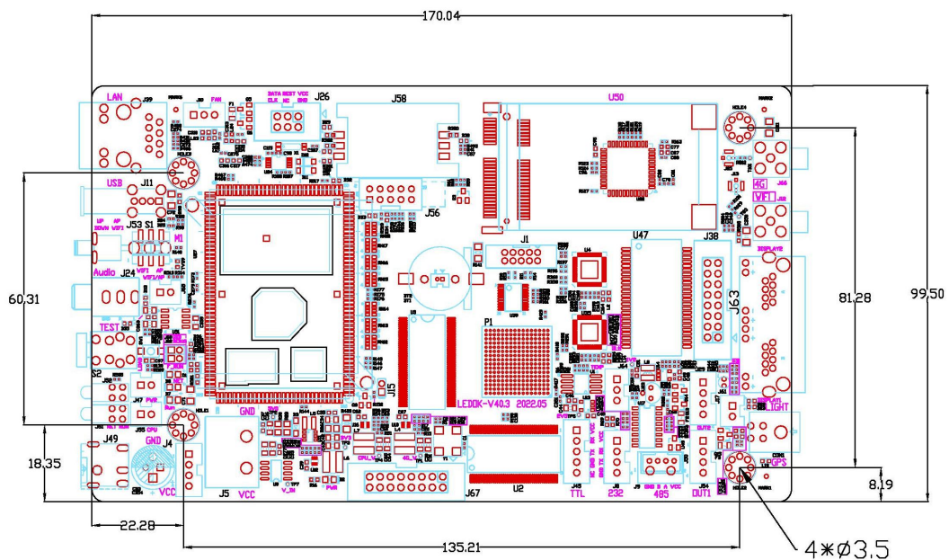
Installation dimensions of bare card M59S
