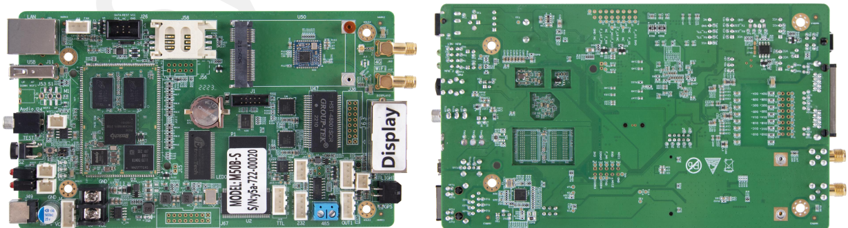
M59S Naked card
